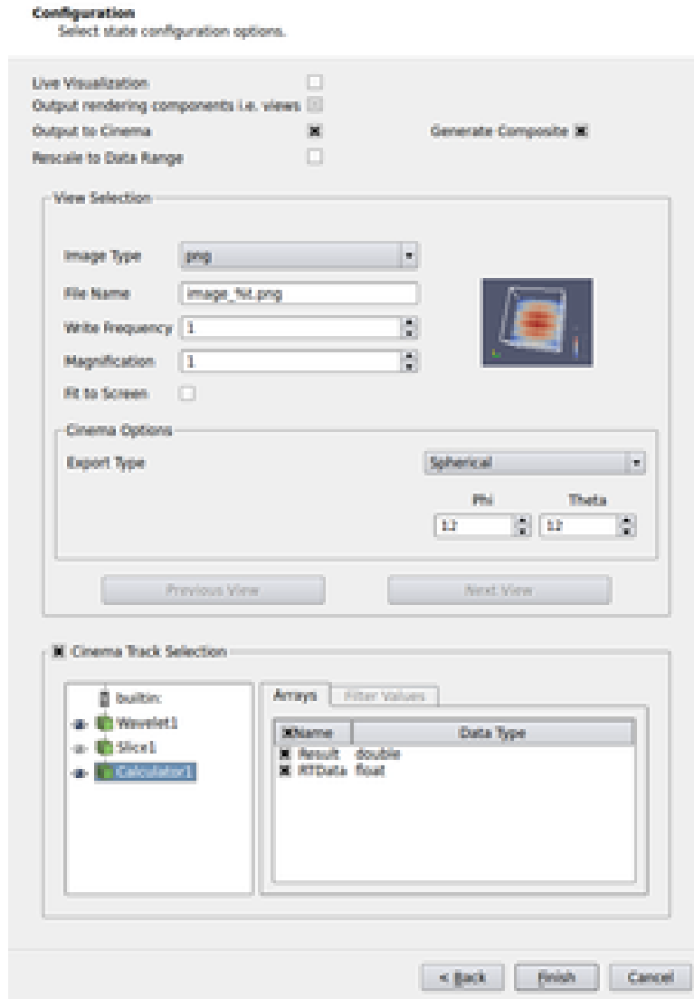
Figure 2.7: ParaView Catalyst export options for Cinema output.
