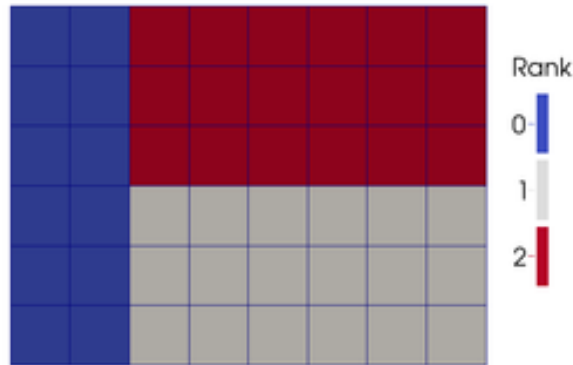
Figure 3.6: Three process partition of a vtkImageData. The whole extent for the points is (0, 8, 0, 6, 0, 0). Process 0 (blue) has an extent of (0, 2, 0, 6, 0, 0) which results in 21 points and 12 cells, process 1 (grey) has an extent of (2, 8, 0, 3, 0, 0) which results in 28 points and 18 cells, and process 2 (red) has an extent of (2, 8, 3, 6, 0, 0) which results in 28 points and 18 cells.
