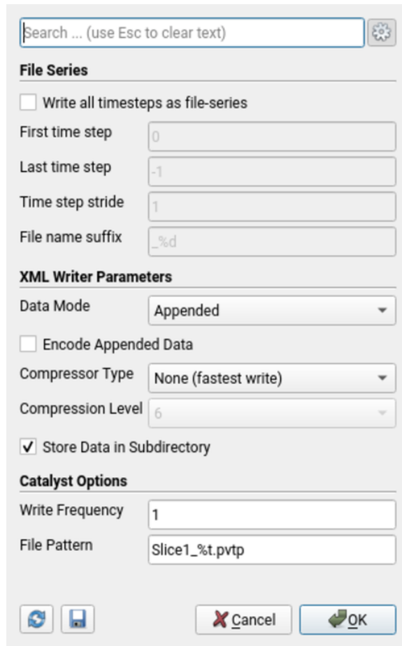
Figure 2.3: Example of a writer options. It writes output from the Slice filter.
