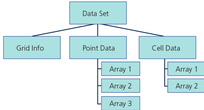
Figure 3.3: High level view of a VTK dataset.
