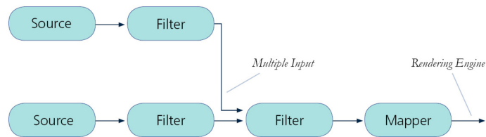
Figure 3.14: VTK Pipeline Example.
