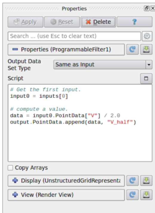
Figure 12.1: Properties panel for Programmable Filter in paraview .
