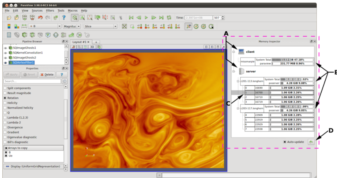
Figure 15.1: The main UI elements of the Memory Inspector panel. A: Process Groups, B: Per-Host statistics, C: Per-Rank statistics, and D: Update controls.
