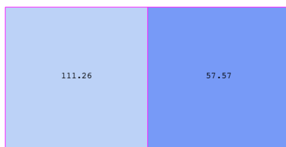
Figure 3.3: Cell-centered attribute.
