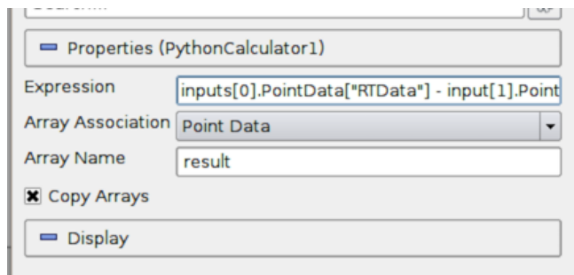
Figure 5.25: The Properties Panel for Python Calculator.
