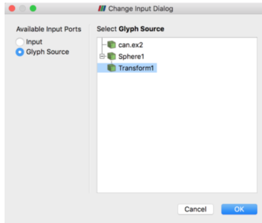
Figure 5.16: Setting the Input and Glyph Source in the Glyph With Custom Source filter.
