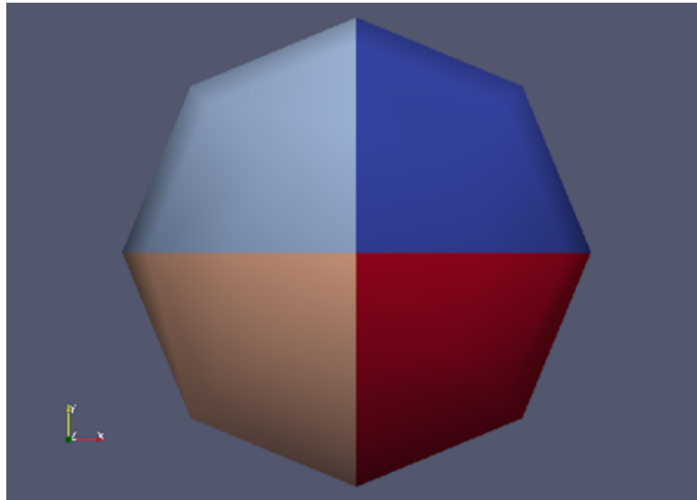
Figure 14.5: Sphere source colored by vtkProcessId array that encodes the processing core on which the sphere data resides. Here, the sphere data is split among the four processing cores invoked by the command mpirun -np 4 pvserver .
