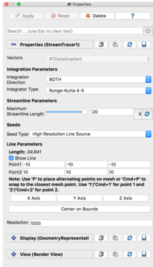
Figure 5.18: The Properties panel showing the default properties for the Stream Tracer filter.
