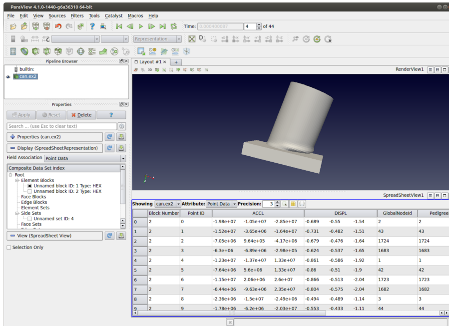
Figure 4.16: paraview using Spreadsheet View to plot raw data values for the can.ex2 dataset.
