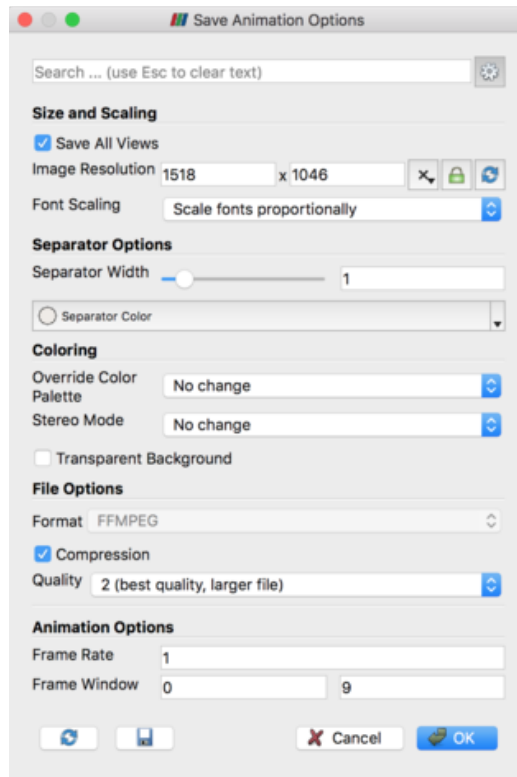
Figure 8.5: The Save Animation Options dialog in paraview , which is used to customize saving of animation.
