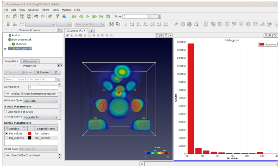
Figure 4.11: paraview using Bar Chart View to plot the histogram for a dataset using the Histogram filter.
