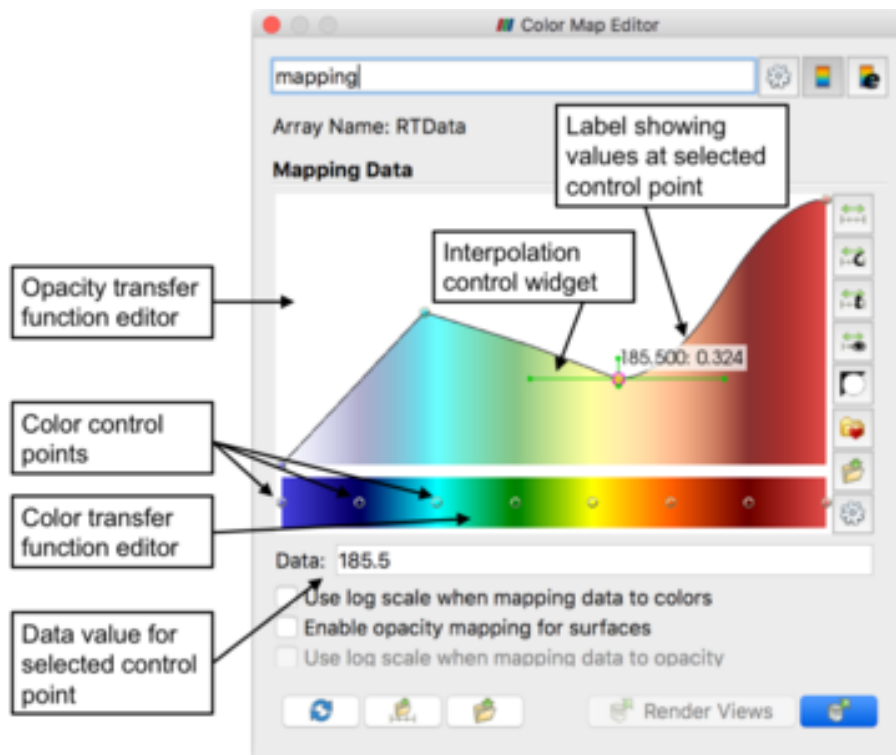
Figure 10.4: Transfer function editor and related properties
