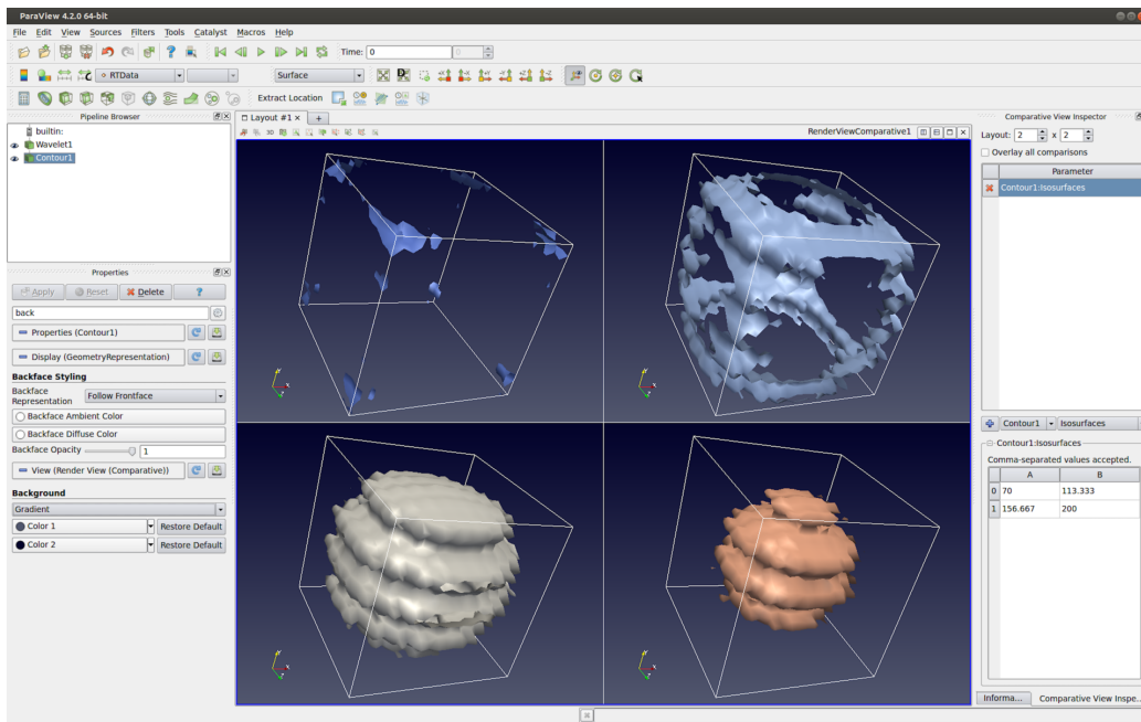
Figure 11.1: Render View (Comparative) in paraview showing a parameter study. In this case, we are comparing the visualization generated using different isovalues for the Contour filter. The Comparative View Inspector dockpanel (on the right) is used to configure the parameter study.
