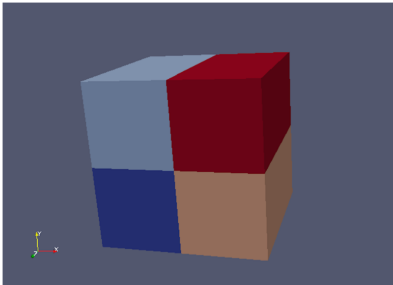
Figure 14.6: Wavelet source processed by the D3 filter and colored by vtkProcessId array. Note how four regions of the image data are split evenly among the four processing cores when pvserver is run with mpirun -np 4 pvserver .
