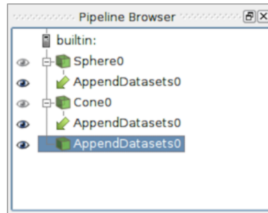
Figure 5.2: The Pipeline Browser showing a pipeline with multiple input connections. The Append Datasets filter has two input connections on its only input port, Sphere0 and Cone0 .
