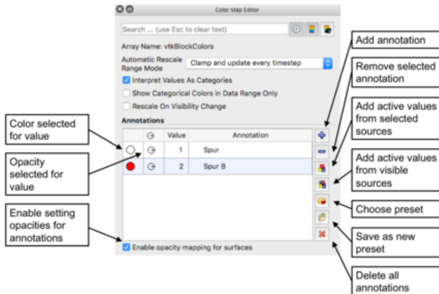
Figure 10.11: Default Color Map Editor when Interpret Values As Categories is checked.
