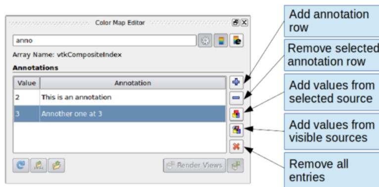
Figure 10.9: Widget to add/edit annotations on the Color Map Editor panel
