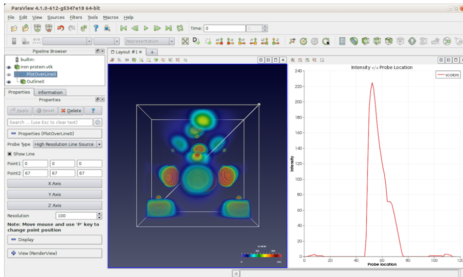
Figure 4.9: paraview using Line Chart View to plot data values probed along a line through the dataset using Plot Over Line filter.
