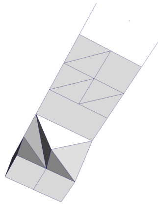
Figure 3.8: Unstructured grid.
