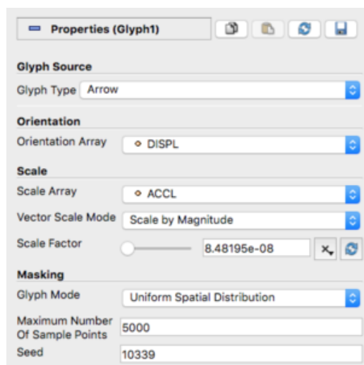
Figure 5.14: The Properties panel for the Glyph filter.
