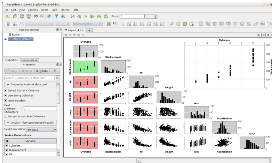
Figure 4.13: paraview using Plot Matrix View to generate a scatter plot matrix to understand correlations between pairs of variables.
