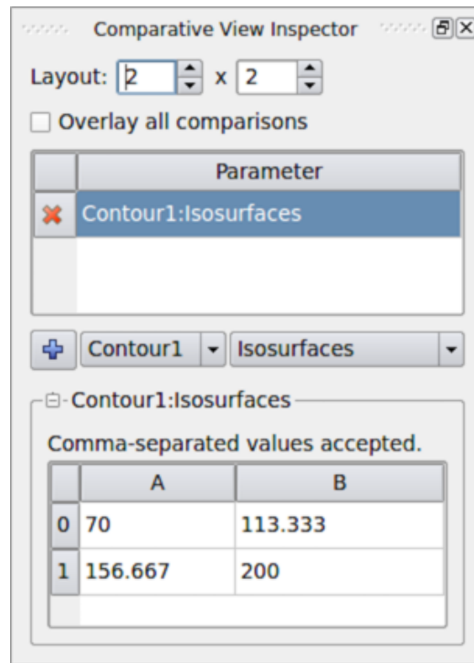
Figure 11.2: Comparative View Inspector in paraview used to configure the active comparative view.
