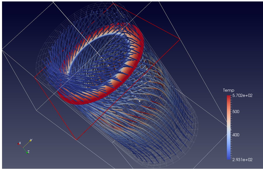
Figure 5.19: Streamlines generated from the disk_out_ref.ex2 dataset using the output of the Slice filter as the Source for seed points.
