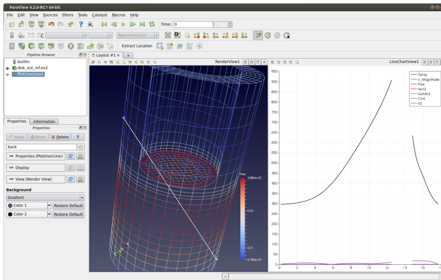
Figure 5.23: The Plot Over Line filter applied to the disk_out_ref.ex2 dataset to plot values at sampled locations along the line. Gaps in the line correspond to the locations in the input dataset where the line falls outside the dataset.
