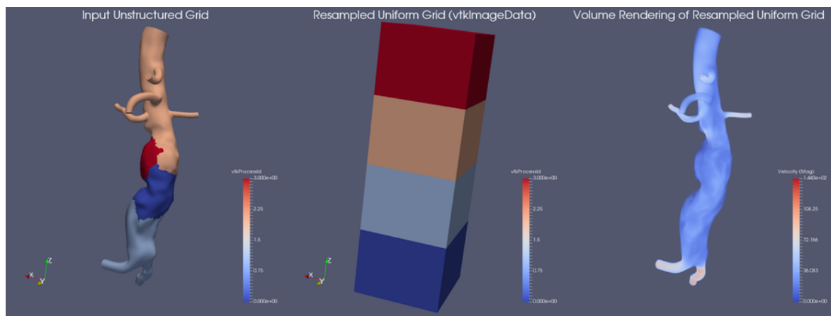
Figure 5.22: An example of Resample To Image. The left portion shows the input (unstructured grid), and the middle displays the output image data. On the right is a volume rendering of the resampled data.
