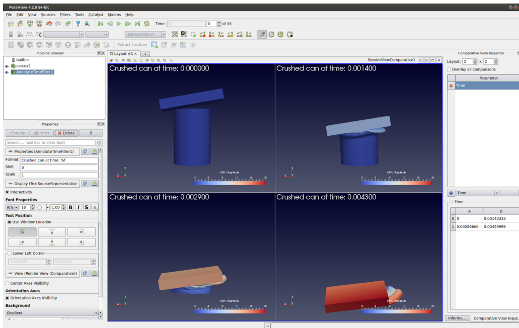
Figure 11.3: Render View (Comparative) with Annotate Time filter showing the time for each of the views. In this case, the parameter study is varying Time across the views.
