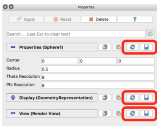
Figure 19.6: Buttons for saving and restoring default property values in the Properties panel.
