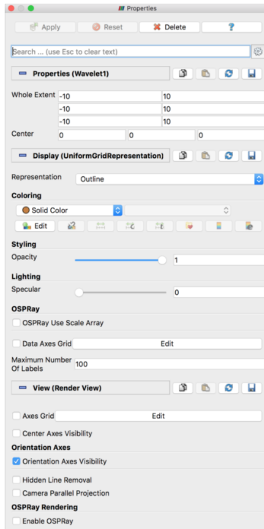
Figure 9.1: Properties Panel in paraview
