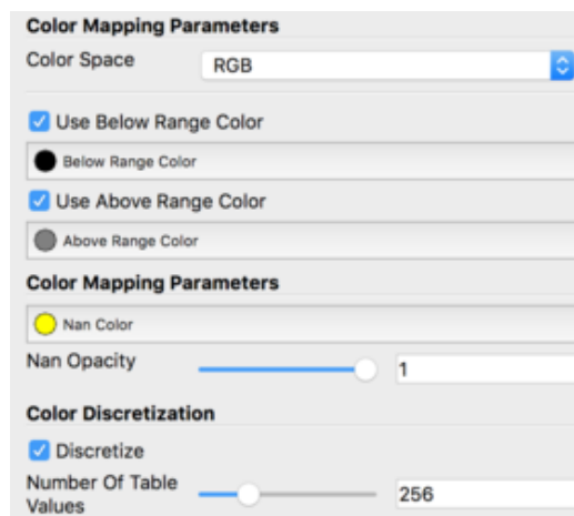
Figure 10.5: Color Mapping Parameters, including advanced properties. Advanced properties are enabled by clicking the gear icon at the top right of the Color Map Editor (not shown).
