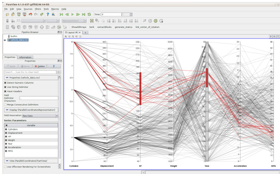
Figure 4.14: paraview using Parallel Coordinates View to plot correlations between columns in a table.
