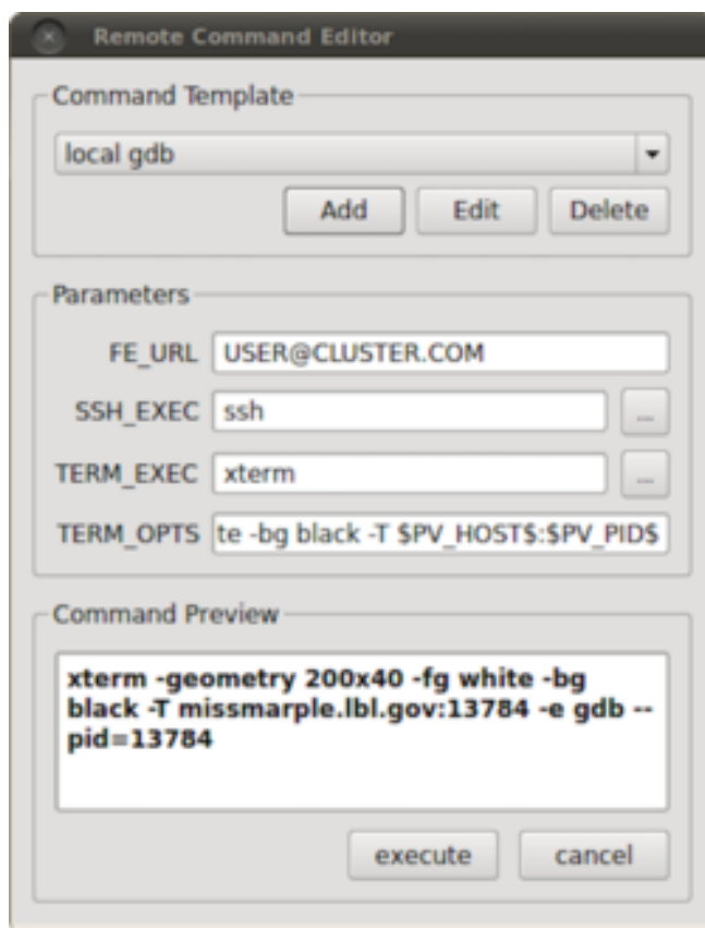
Figure 15.3: The remote command dialog.
