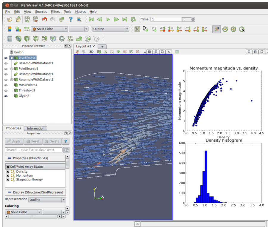
Figure 4.18: paraview using Python View with matplotlib to display a scatterplot of momentum magnitude versus density (upper right) and a histogram of density (lower right) in the bluntnfin.vts dataset.
