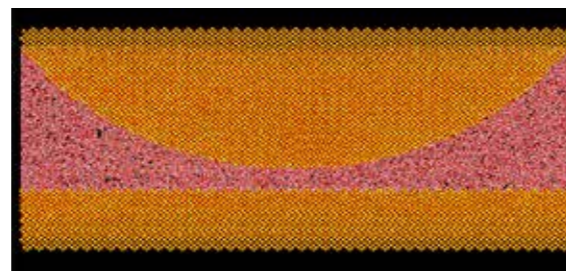
Fig. 4: Picture from initial workshop with summer students; Illustration from simulations of a silicate nano-indentor in water by Anders Johansson.
