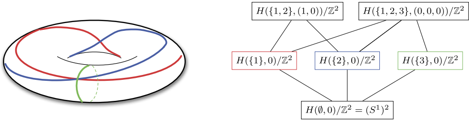
Fig. 4. Left-hand side: a drawing of the toric arrangement \underline{\mathcal{A}} associated to the periodic line arrangement \mathcal{A} of Example 2.1. Right-hand side: the poset of layers \mathcal{C}(\underline{\mathcal{A}}) .
